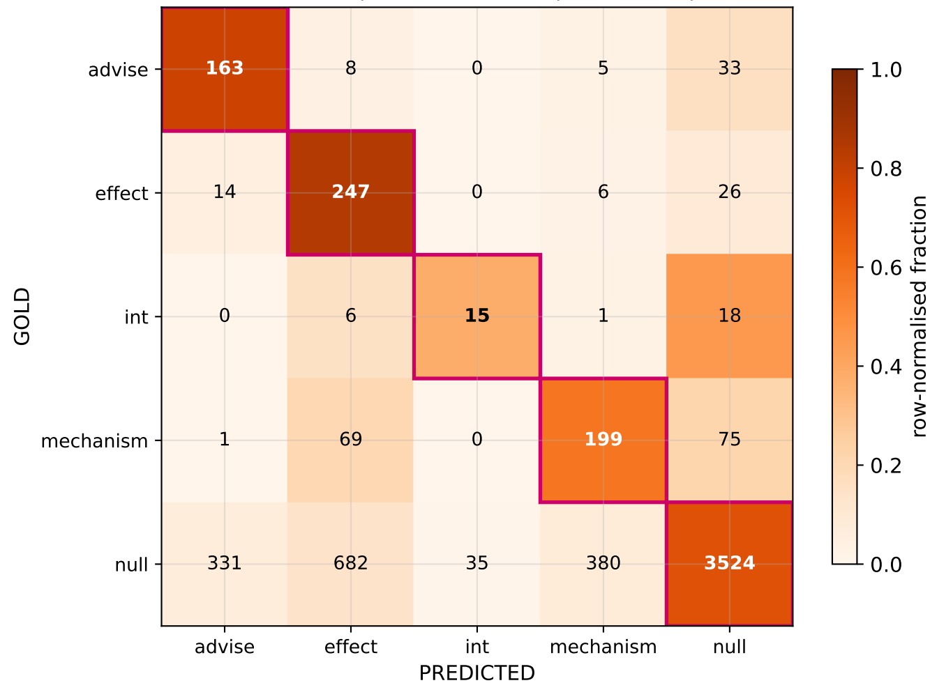
Confusion matrix — champion Llama r=32 / prompts02 (test) 1428 / 4952 null pairs (28.8%) over-predicted as positive
