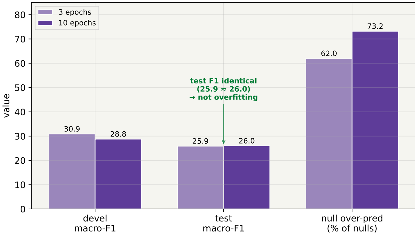
Qwen prompts02 epoch ablation — the over-prediction collapse is present at epoch 3; more epochs only raise over-prediction, not F1
