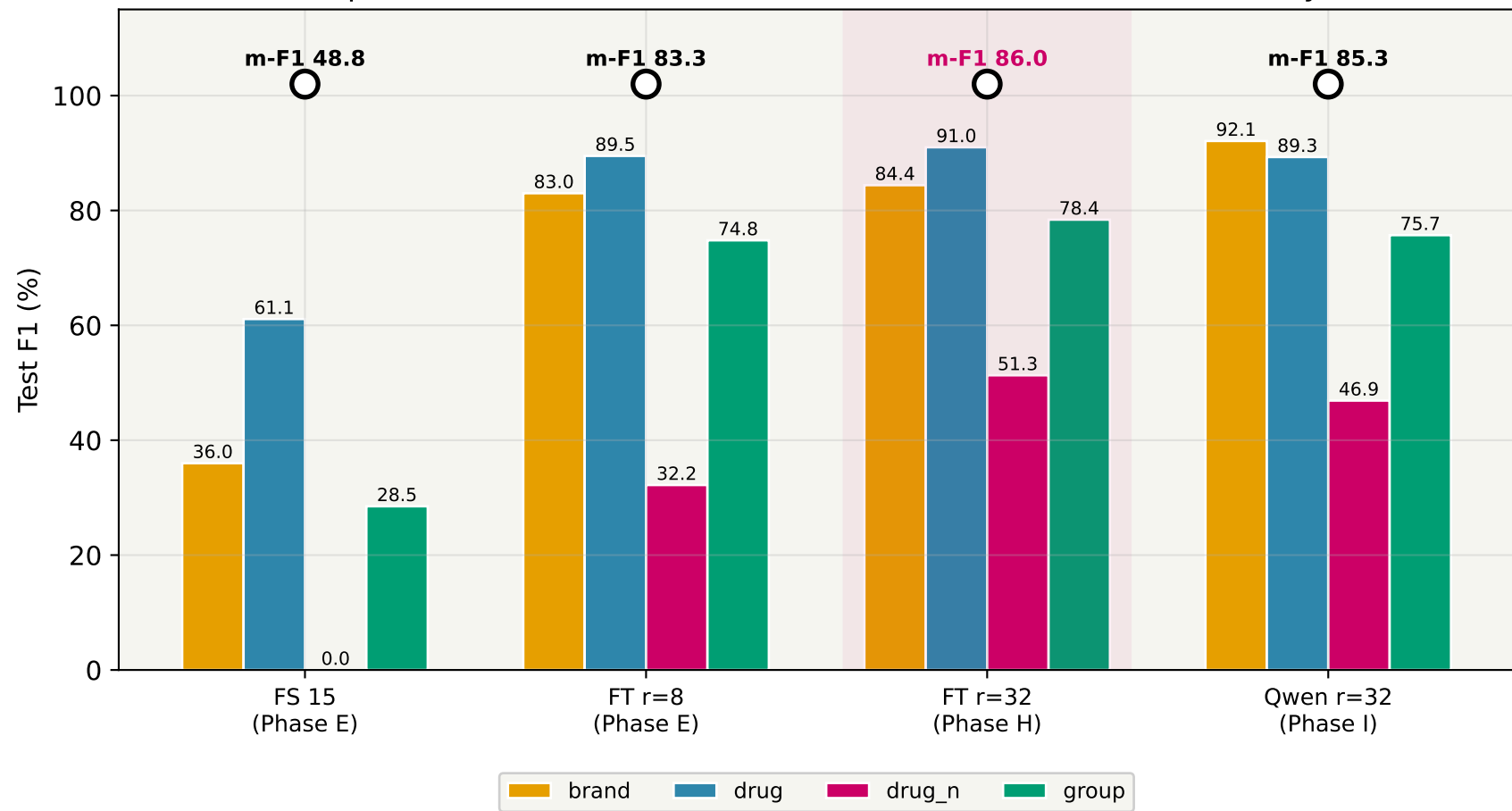
Test-set per-class F1 — final head-to-head between our four test-run systems
