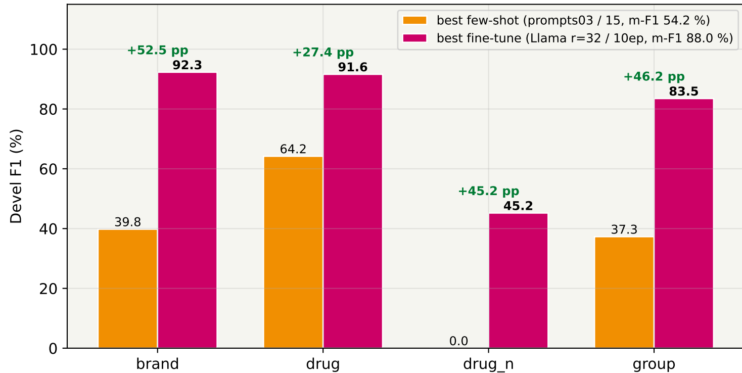
Few-shot → fine-tune gains per class (same base model, same 4-bit quant)
