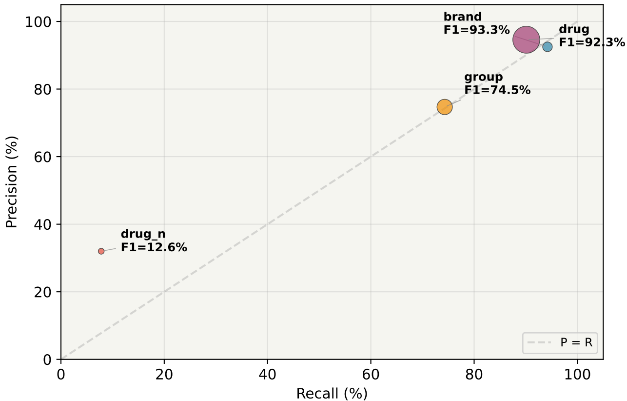
Precision vs Recall per Entity Type (Best CRF, mod8, Test Set)
