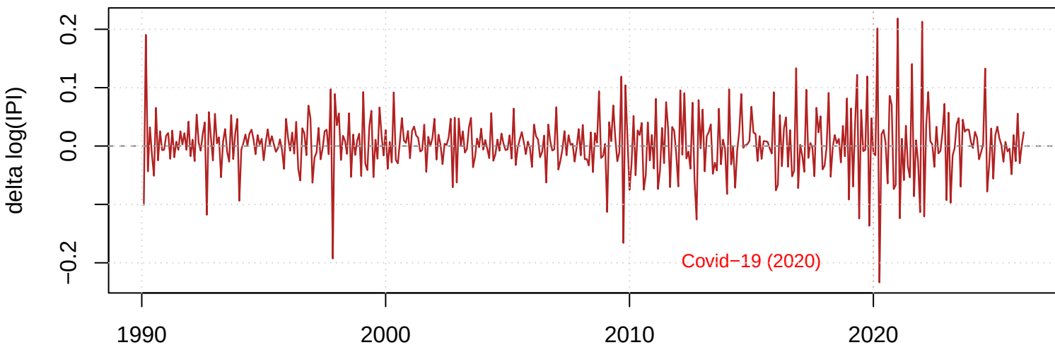
Stationary series: delta log(IPI)
