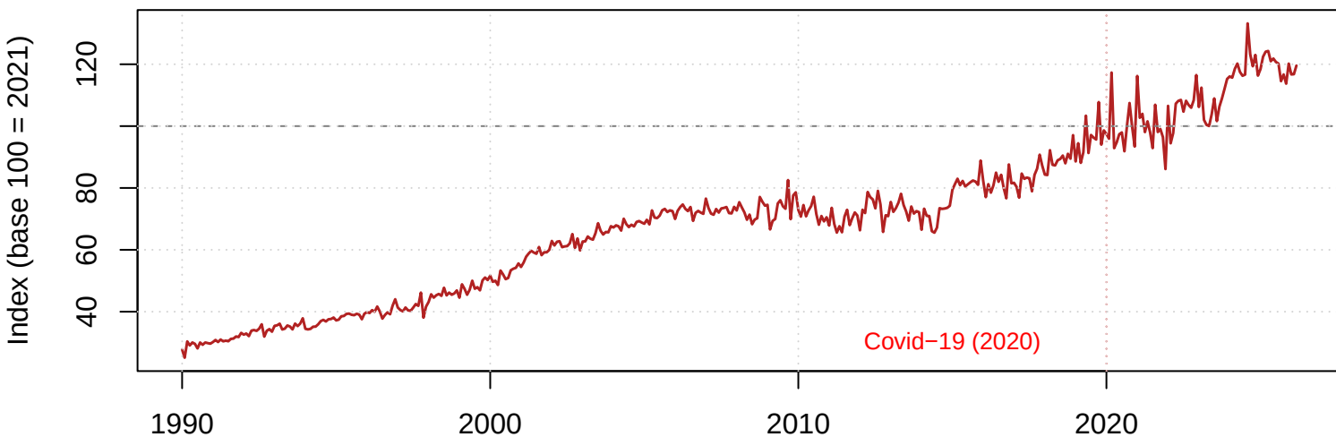
Raw series: IPI Pharmaceutical industry (NAF 21)
