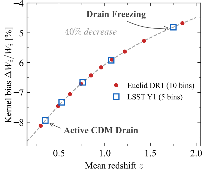
FIG. 5. Kernel bias gradient \Delta W_i/W_i as a function of mean tomographic redshift for Euclid DR1 (10 bins, circles) and LSST Y1 (5 bins, squares). The 40% decrease from \bar{z} \approx 0.3 to \bar{z} \approx 1.8 traces the CDM drain freezing at high redshift.
