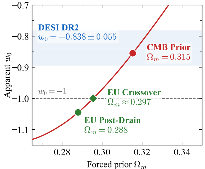
FIG. 6. The CPL mirage: apparent w_0 recovered by a w CDM pipeline as a function of the forced \Omega_m prior. The EU predicts w_0 = -0.855 at \Omega_m = 0.315 (red circle), consistent with the DESI DR2 measurement w_0 = -0.838 \pm 0.055 (blue band) at 0.3\sigma . Crossover w_0 = -1 at \Omega_m \approx 0.297 (green diamond).
