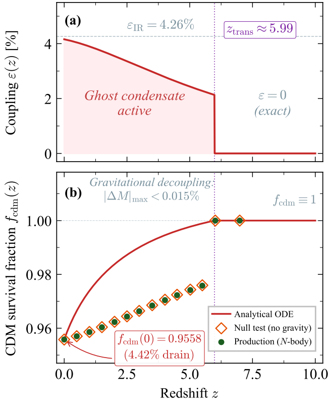
FIG. 2. Anatomy of the evaporating universe. (a) The coupling function \varepsilon(z) , with logistic activation at z_{\text{trans}} \approx 5.99 and IR plateau \varepsilon_{\text{IR}} = 4.26\% . (b) CDM survival fraction f_{\text{cdm}}(z) : analytical solution (solid), N -body snapshots (circles), and null-test particles (diamonds).
