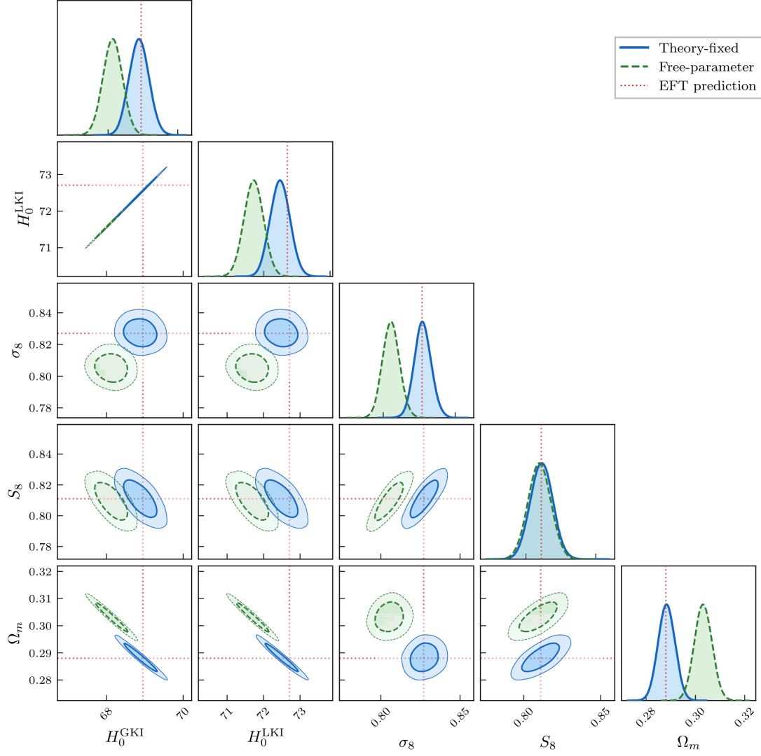
FIG. 7. Posterior comparison between the theory-fixed configuration (blue) and the EU-blind free-parameter configuration (green). Diagonal panels show 1D marginalized posteriors; off-diagonal panels show 68% and 95% credible regions. Red dotted lines mark the framework-derived values.
