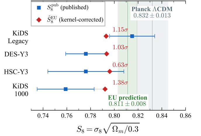
FIG. 4. Resolution of the growth tension across four independent Stage-III weak-lensing surveys. For each survey, the published S_8^{\text{pub}} (extracted under \Lambda\text{CDM} assumptions) is compared with the EU forward-model prediction \hat{S}_8 . The kernel bias shifts all surveys toward concordance with the CMB, reducing the average tension from \sim 2.6\sigma to \sim 1\sigma .
