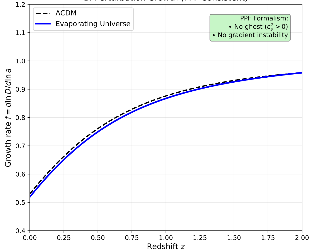
B. Perturbation Growth (PPF Consistent)
