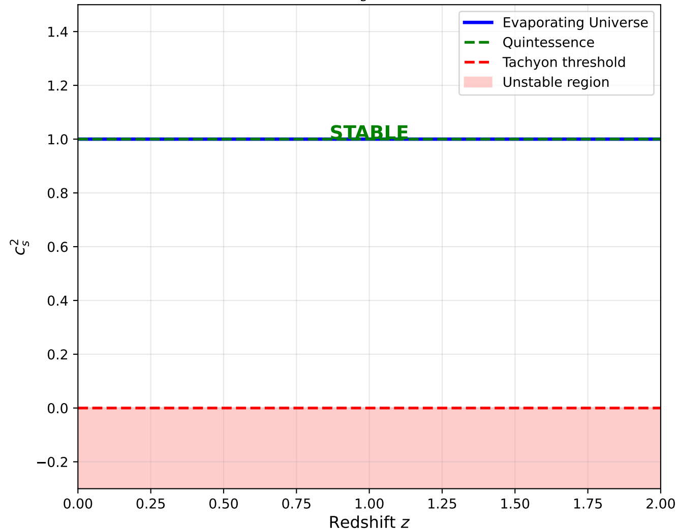
A. Sound Speed: c_s^2 \geq 0 (Tachyon-free)
