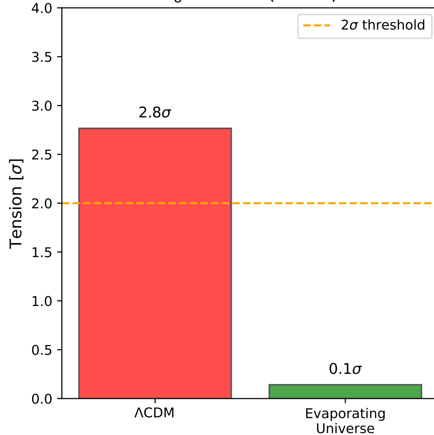
S_8 Tension (vs WL)
