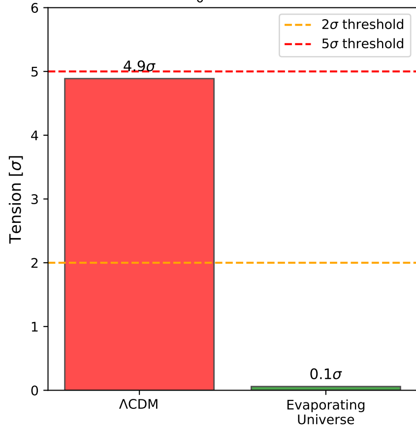
H_0 Tension
