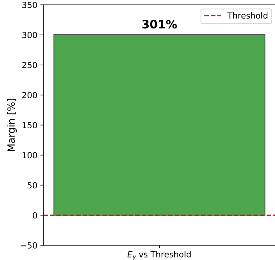
Li-7 BBN Resolution
