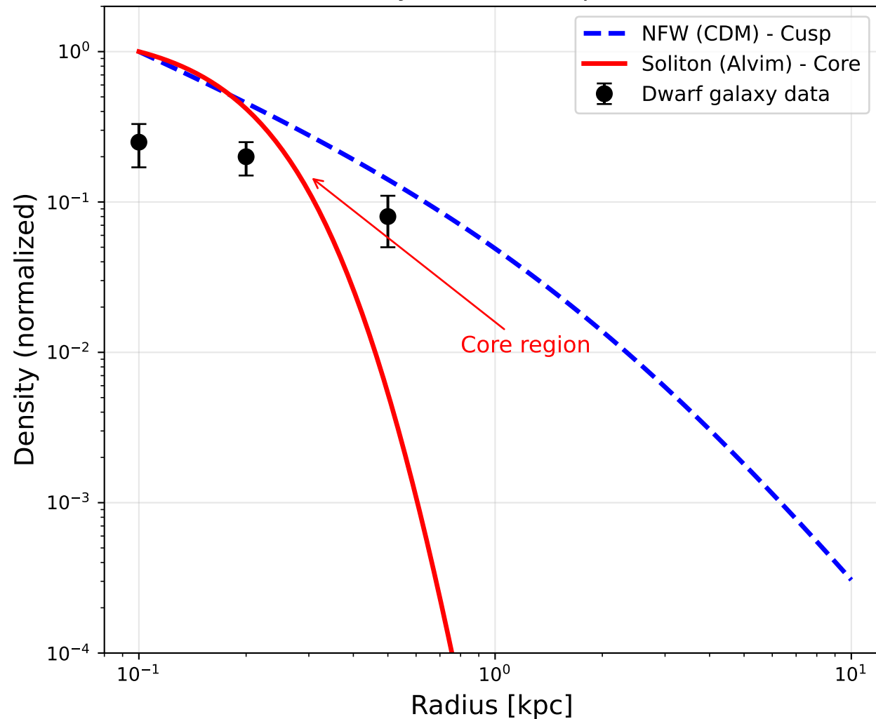
A. Density Profiles: Cusp vs Core
