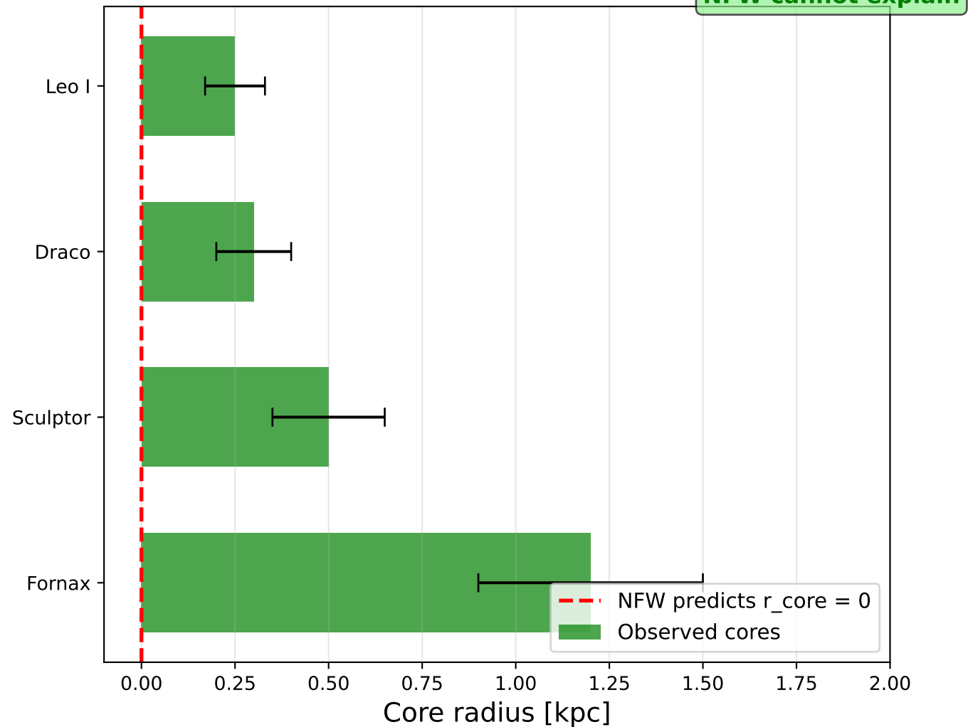
B. Observed Cores in Dwarf Galaxies
