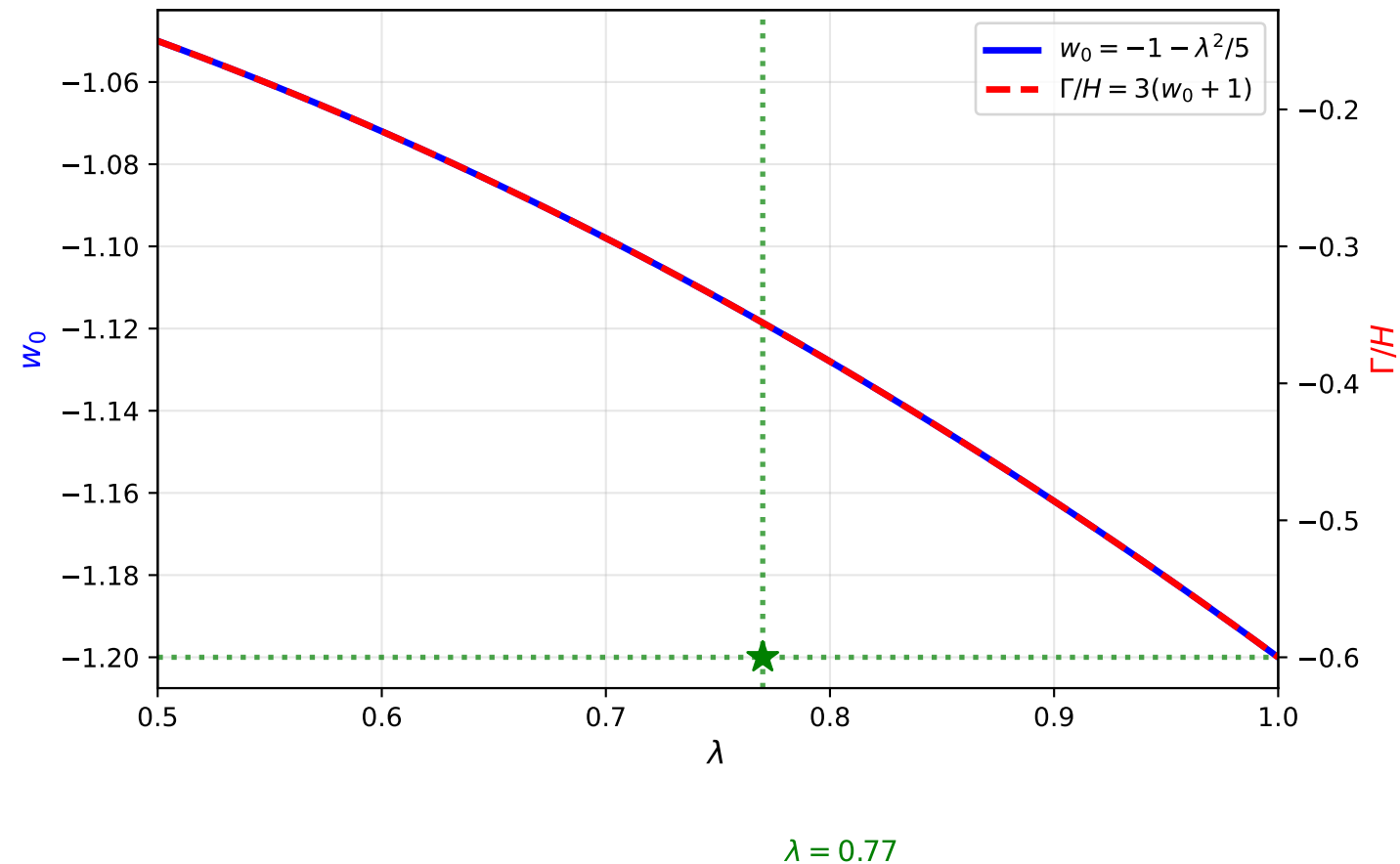
C. Derivation Chain: \lambda \rightarrow w_0 \rightarrow \Gamma/H
