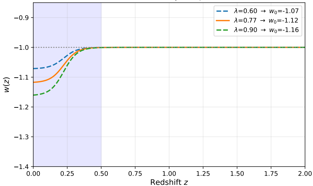
A. w(z) from V(\phi) = V_0 e^{\lambda \phi/M_{pl}}
