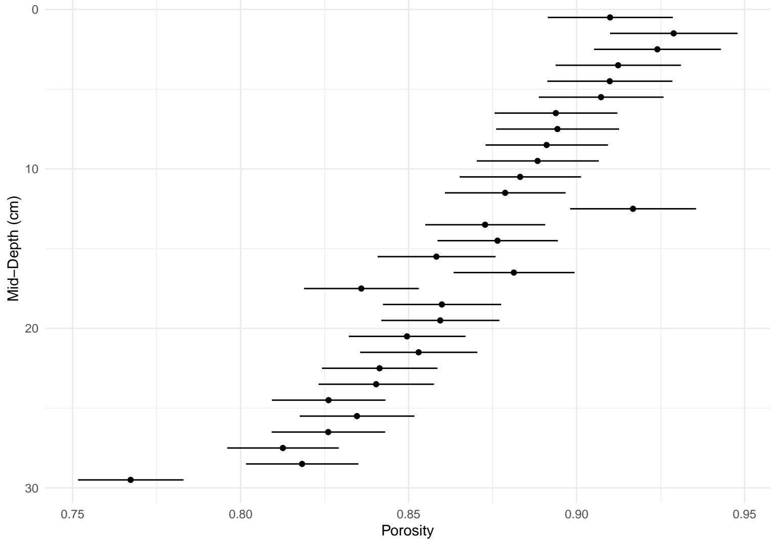
Porosity verses Depth
