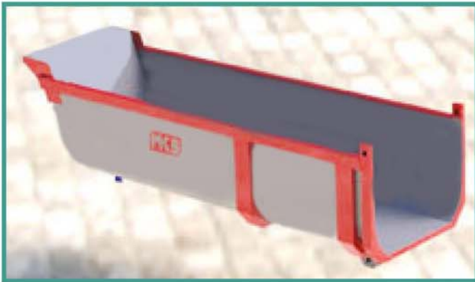
Tipper Truck Hardox 450 HBW Size/ 2.6Mx9.30M-Capacity / 32M 3
