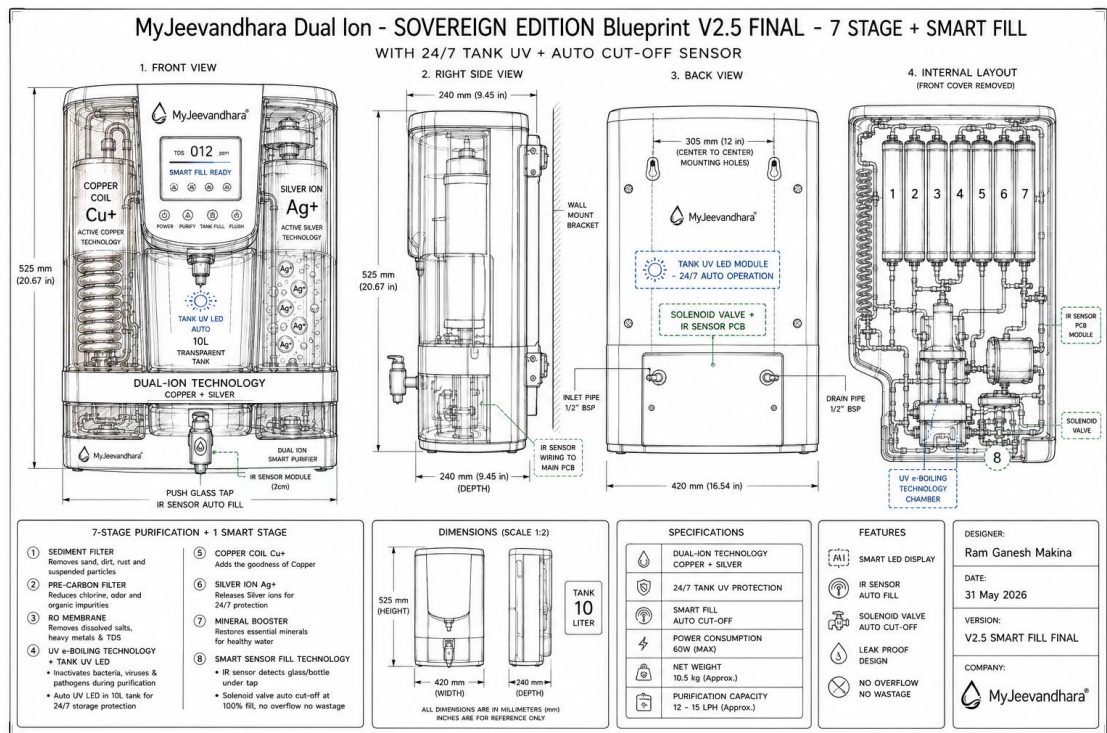
Figure 2. MyJeevandhara Dual Ion Sovereign Edition Blueprint
