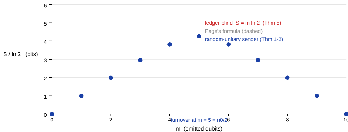
Figure 1. The evaporation ledger, n_0 = 10 qubits
