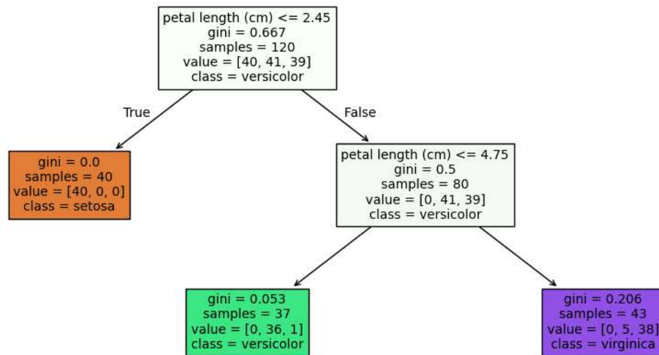
Iris Decision Tree (max_depth=2)
