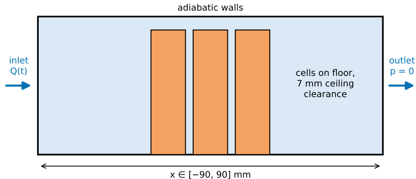
(b) production duct, 180 × 46 × 72 mm
