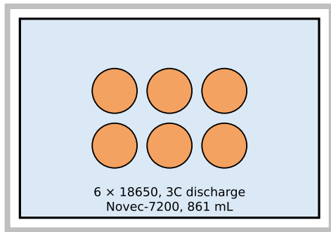
(a) validation rig: static immersion
