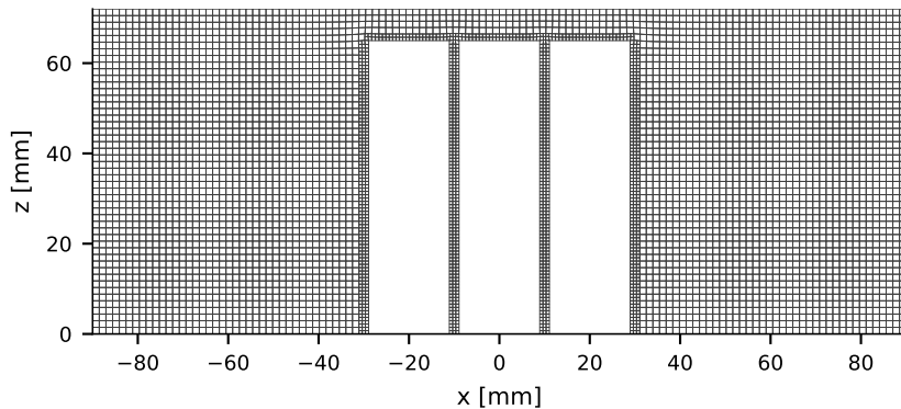
(b) vertical plane through one cell row, y = 11 mm
