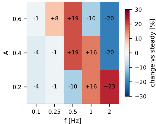
(b) cell-to-cell \sigma_T change [%]
