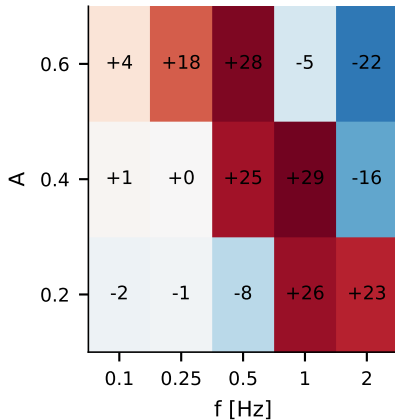
(a) module \Delta T change [%]
