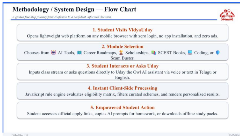
Figure 4.2: End-to-End User Guidance & Decision Tree Flowchart
