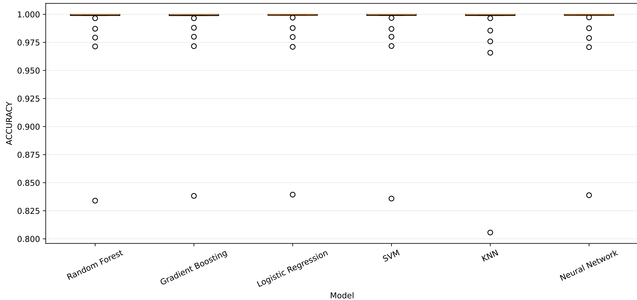
ACCURACY distribution across experiments
