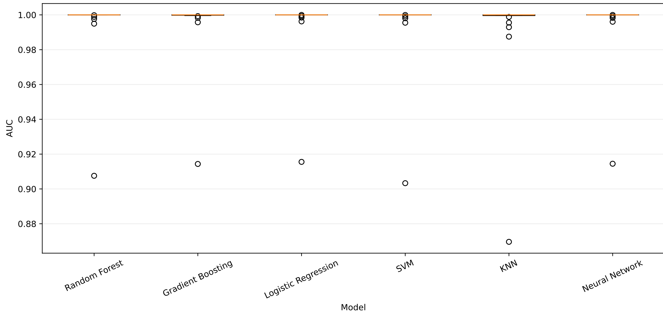
AUC distribution across experiments
