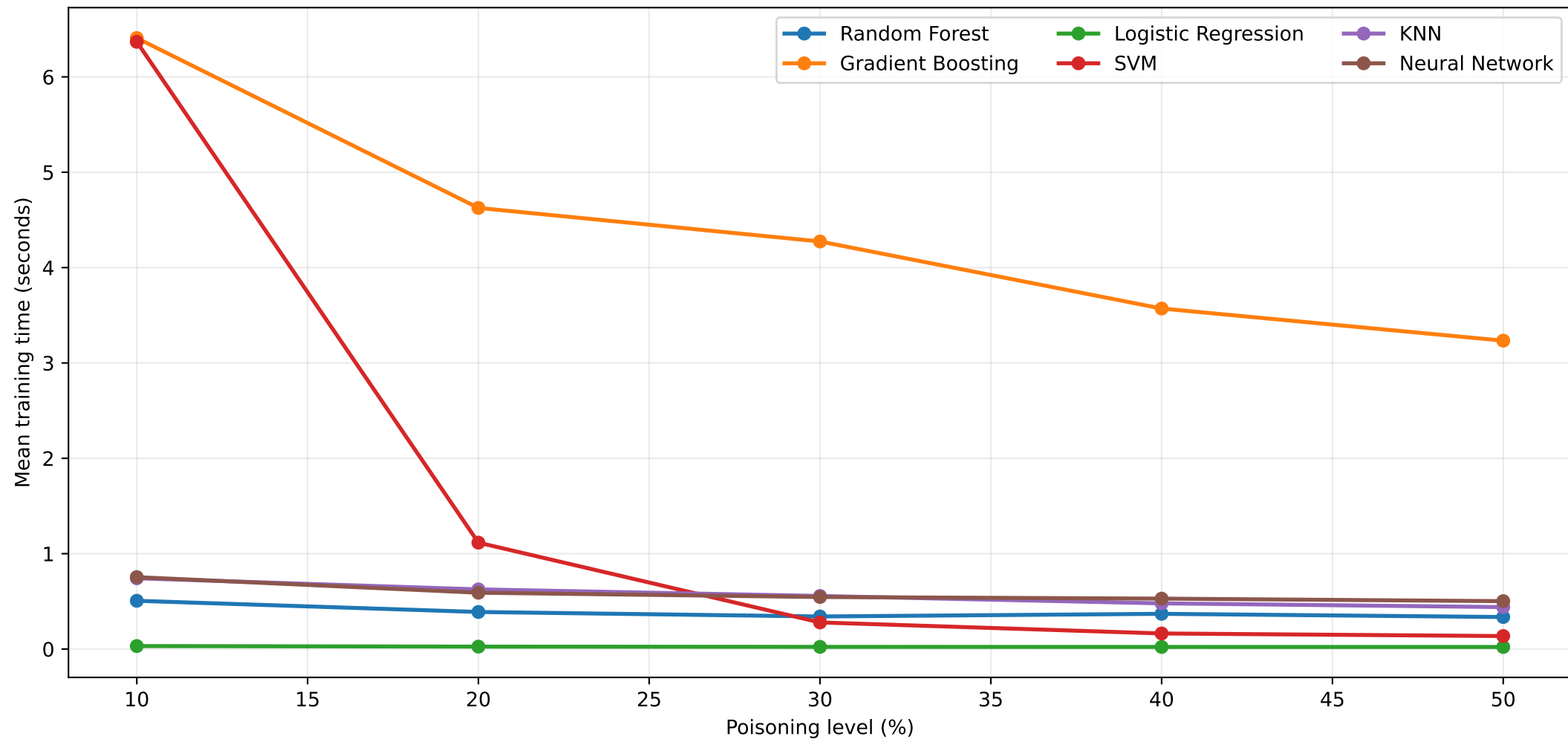
Training time by poisoning level
