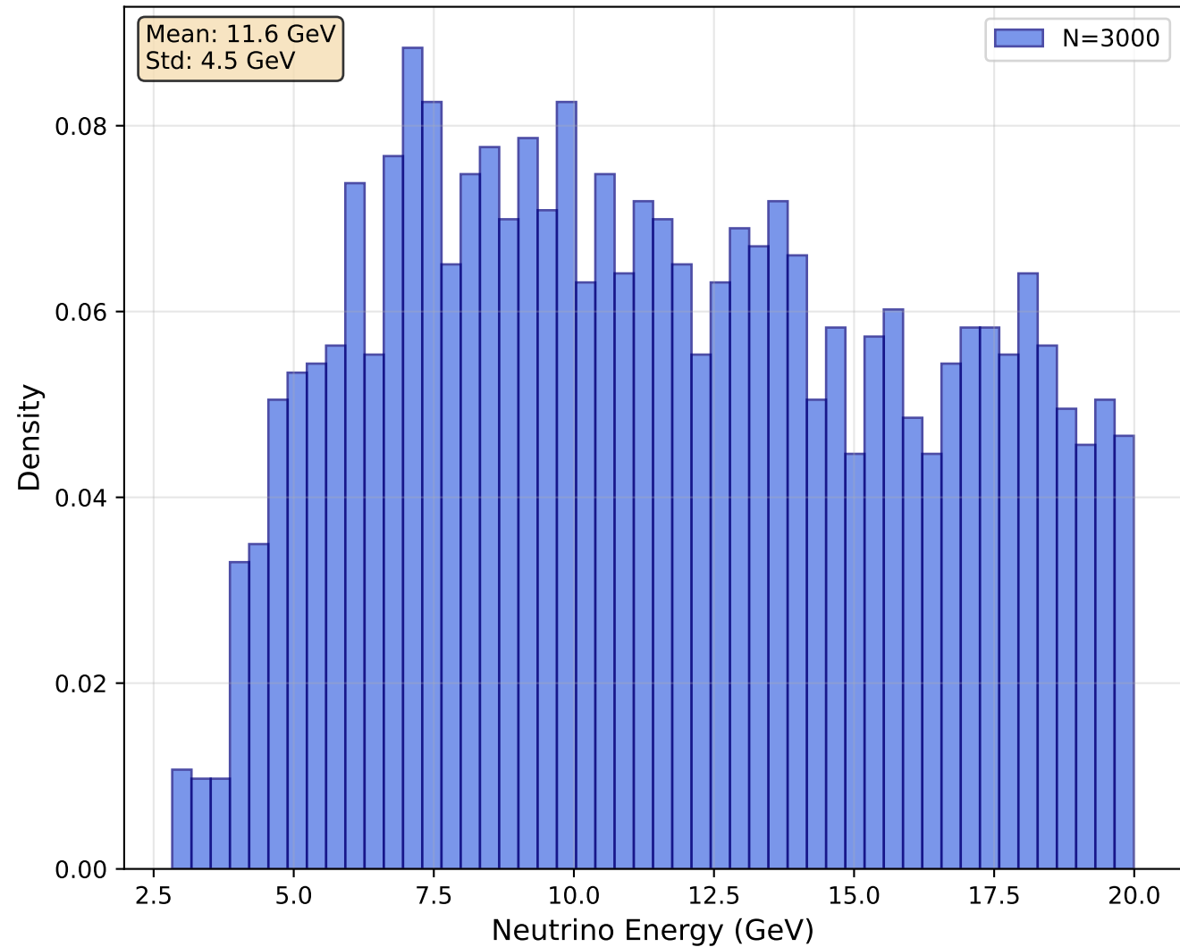
Neutrino Energy Distribution
