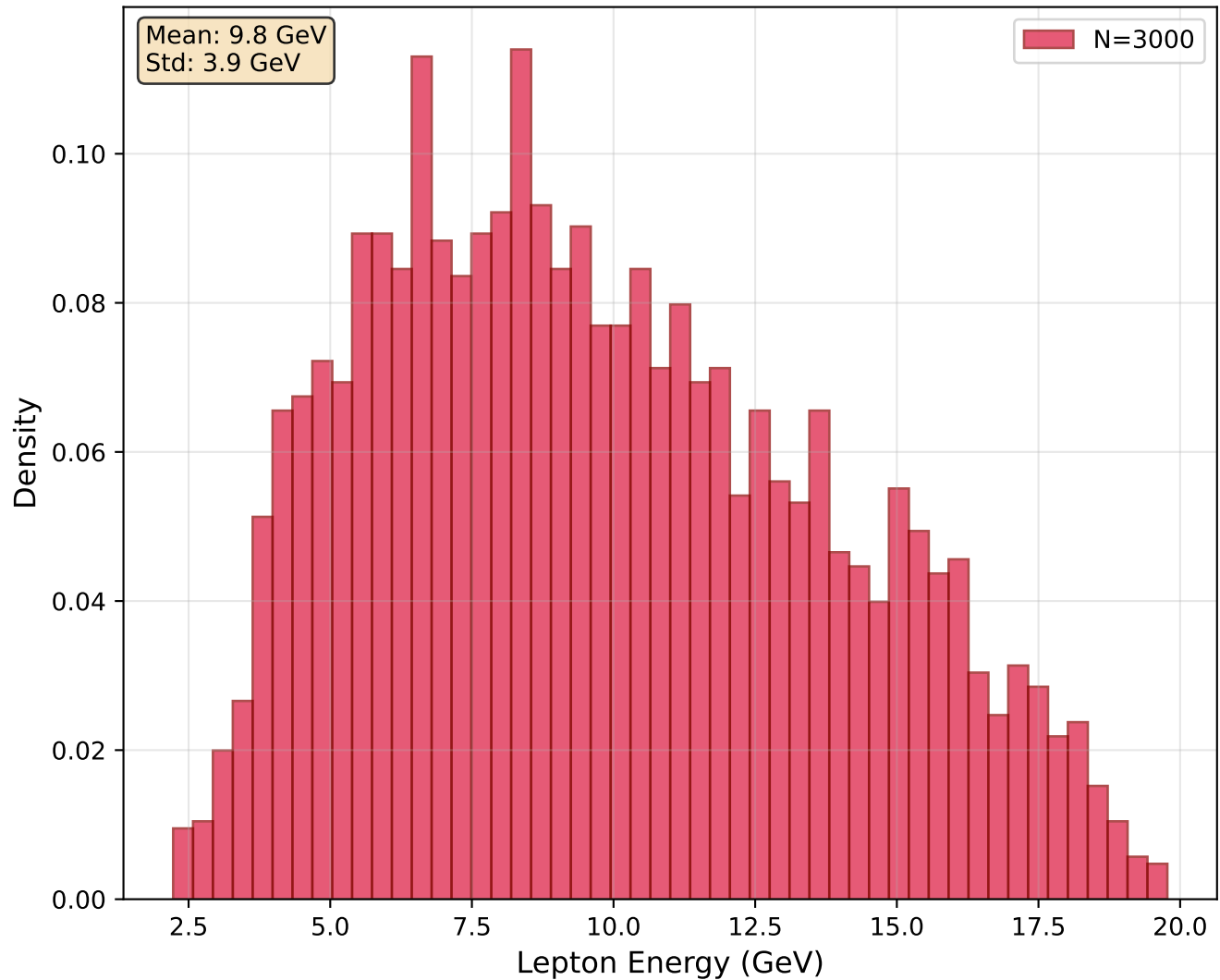
Lepton Energy Distribution
