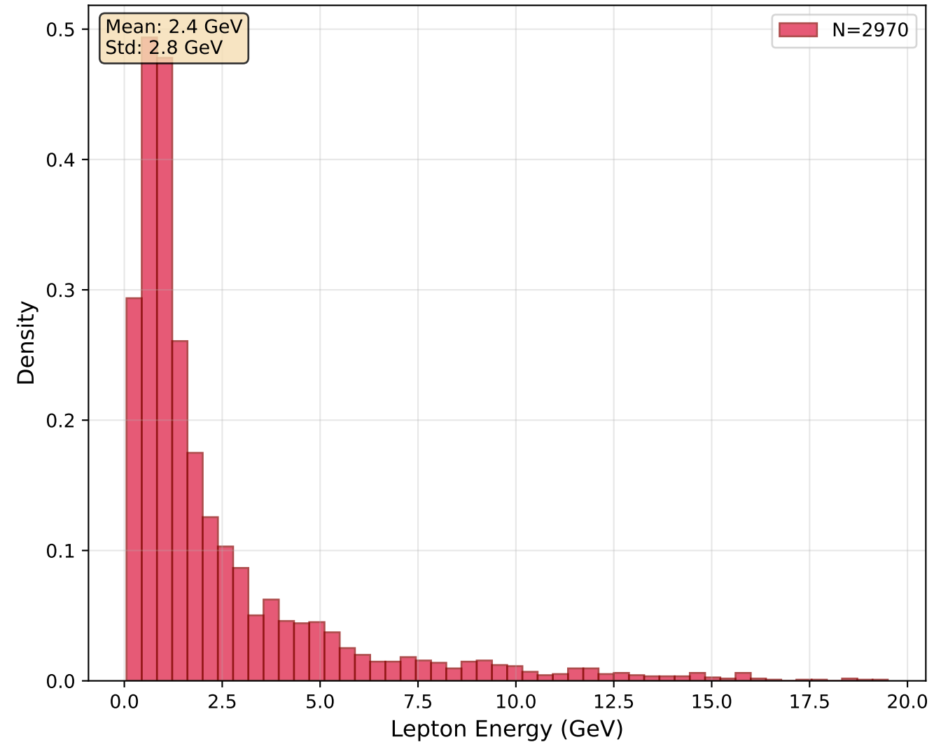
Lepton Energy Distribution
