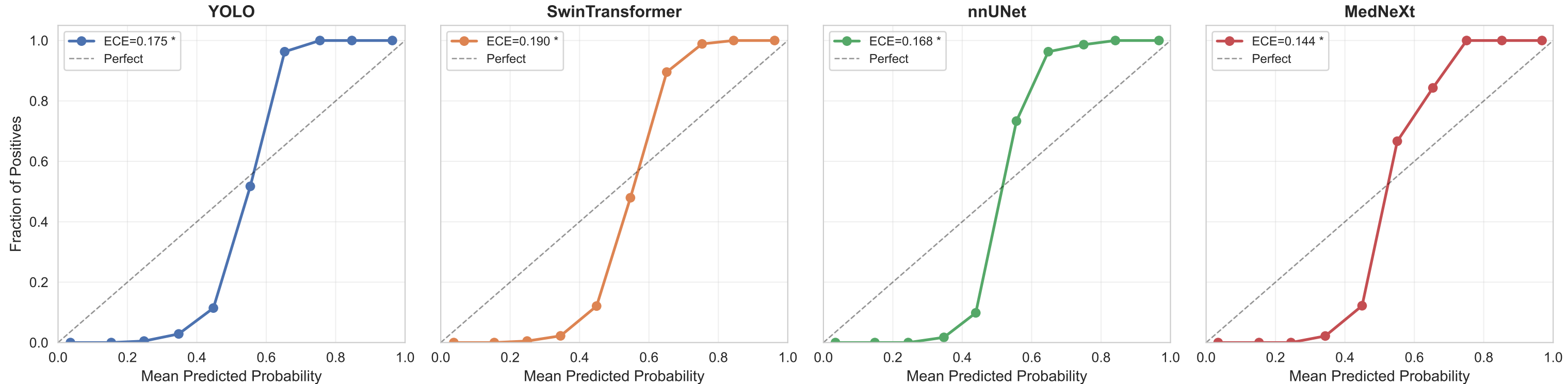
Figure 10 — Reliability Diagrams (Calibration)
