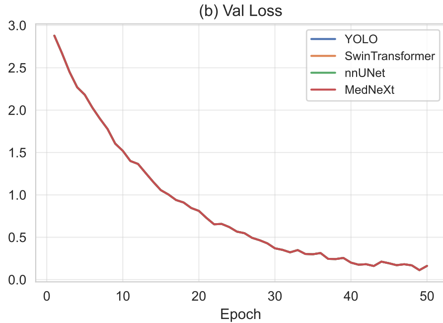
Figure 2 — Training Curves
