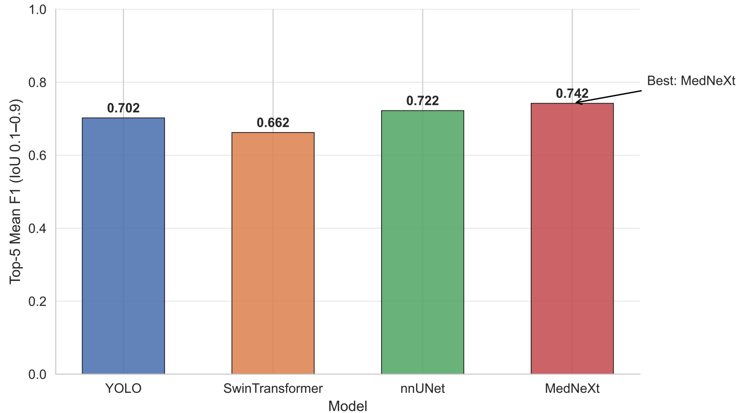
Figure 3 — Model Comparison: Top-5 Mean F1
