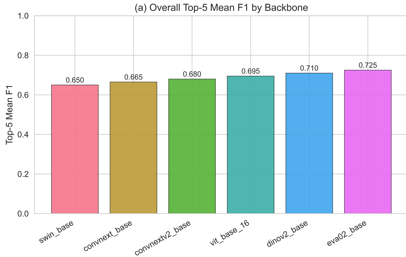
Figure 5 — Backbone Ablation Study
