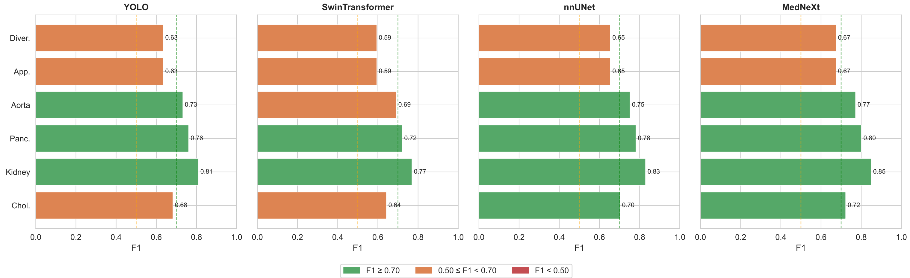
Figure 6 — Per-Class F1 Error Analysis by Model
