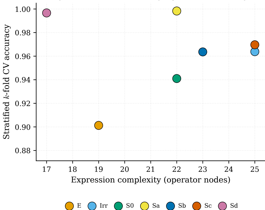
Symbolic head: accuracy against complexity
