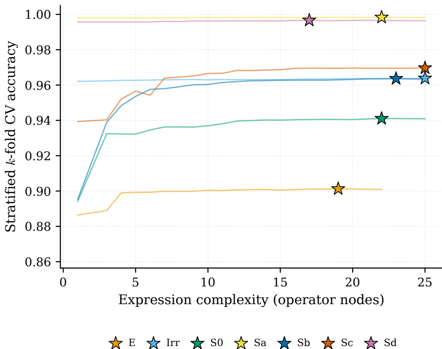
Symbolic head: accuracy against complexity lines : PySR Pareto front; stars : adopted rule
