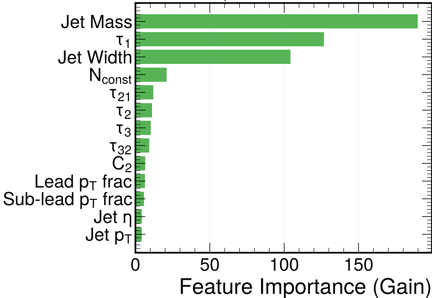
BDT Feature Importance: Jet Substructure Variables
