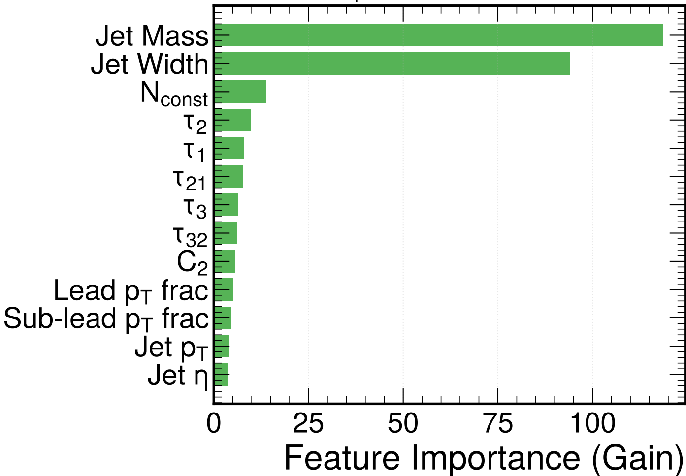
BDT Feature Importance: Jet Substructure Variables
