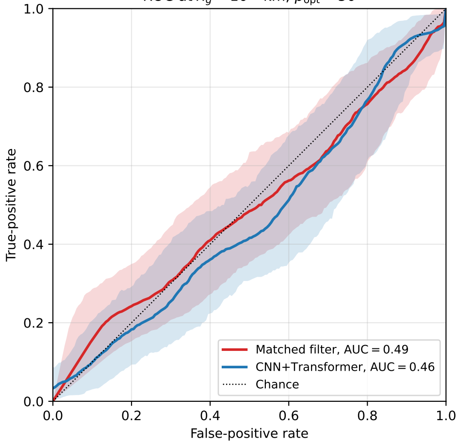
ROC at \lambda_g = 10^{12} km, \rho_{\text{opt}} = 50
