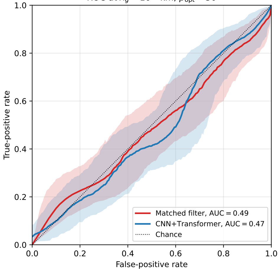
ROC at \lambda_g = 10^{14} km, \rho_{\text{opt}} = 50
