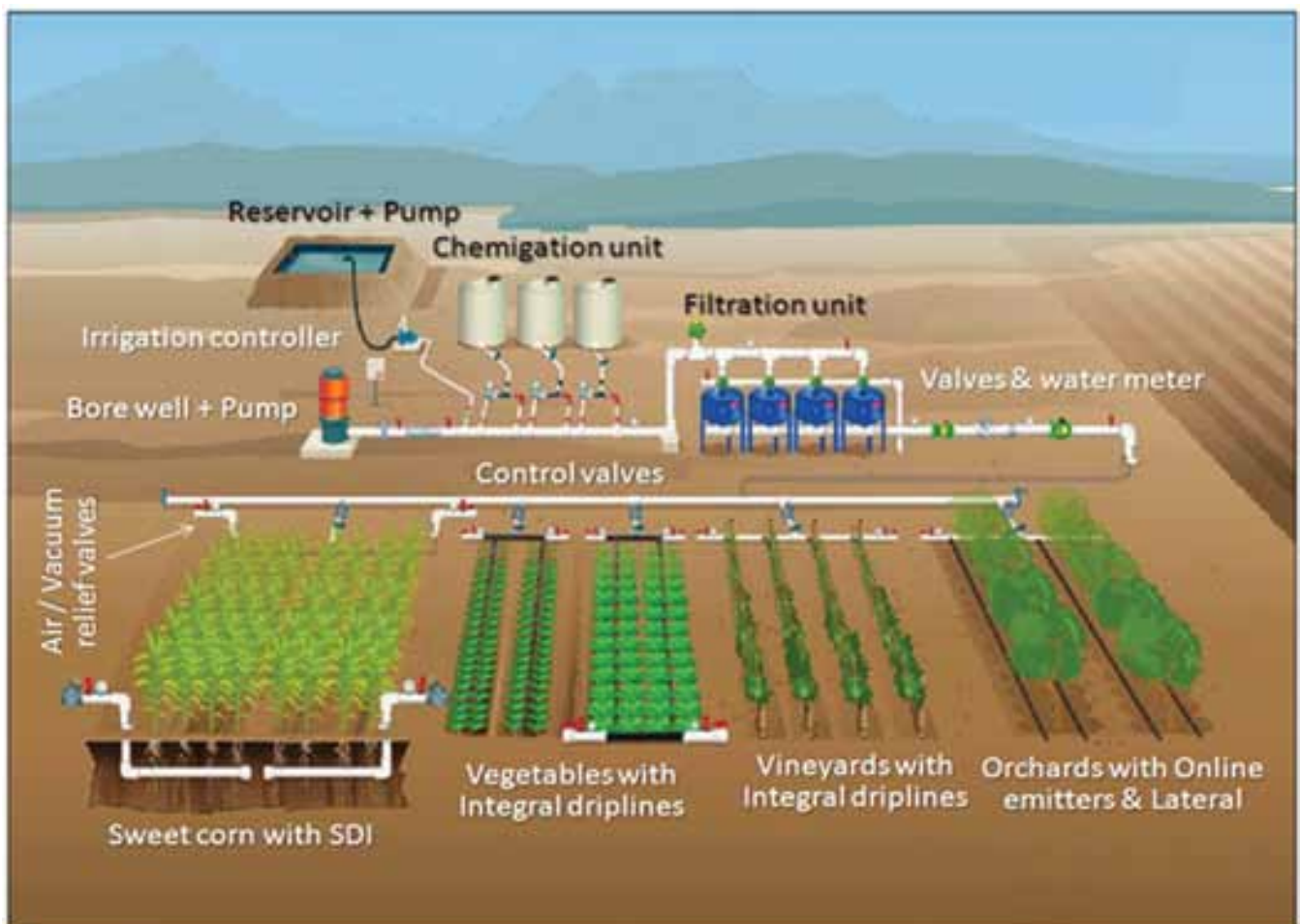
Photo 4: Working of Drip Irrigation System
