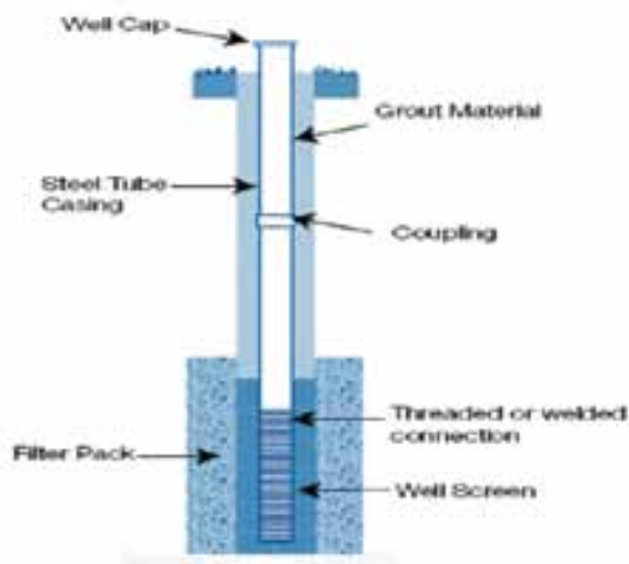
Photo 13: Design of Shallow Tube Well
