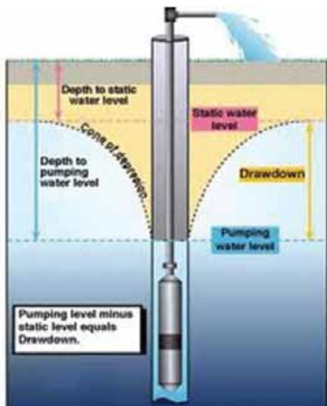
Photo 16: Working of Deep Tube well
