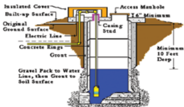
DUG WELL
