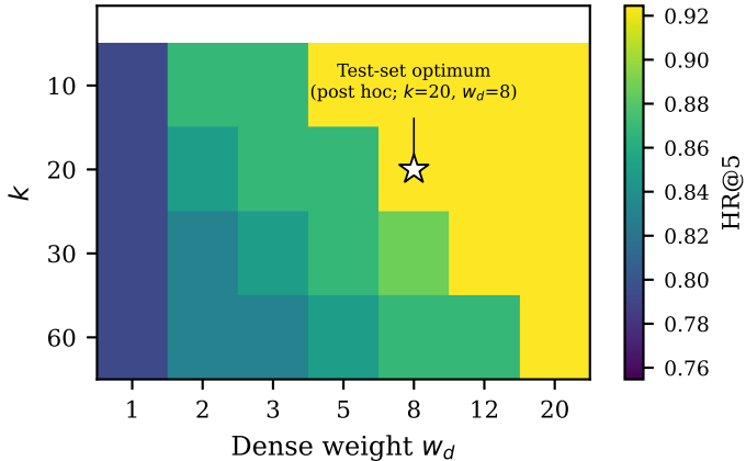
Test-set optimum's slice (top- k_r=20 )
