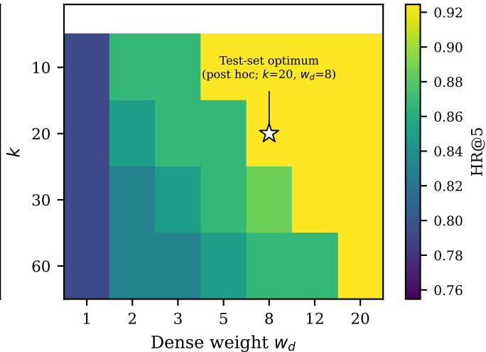
Test-set optimum's slice (top- k_r=20 )
