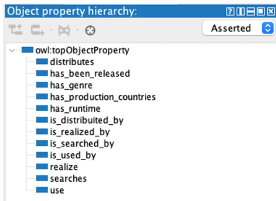
Figura 4-2: Object-Properties
