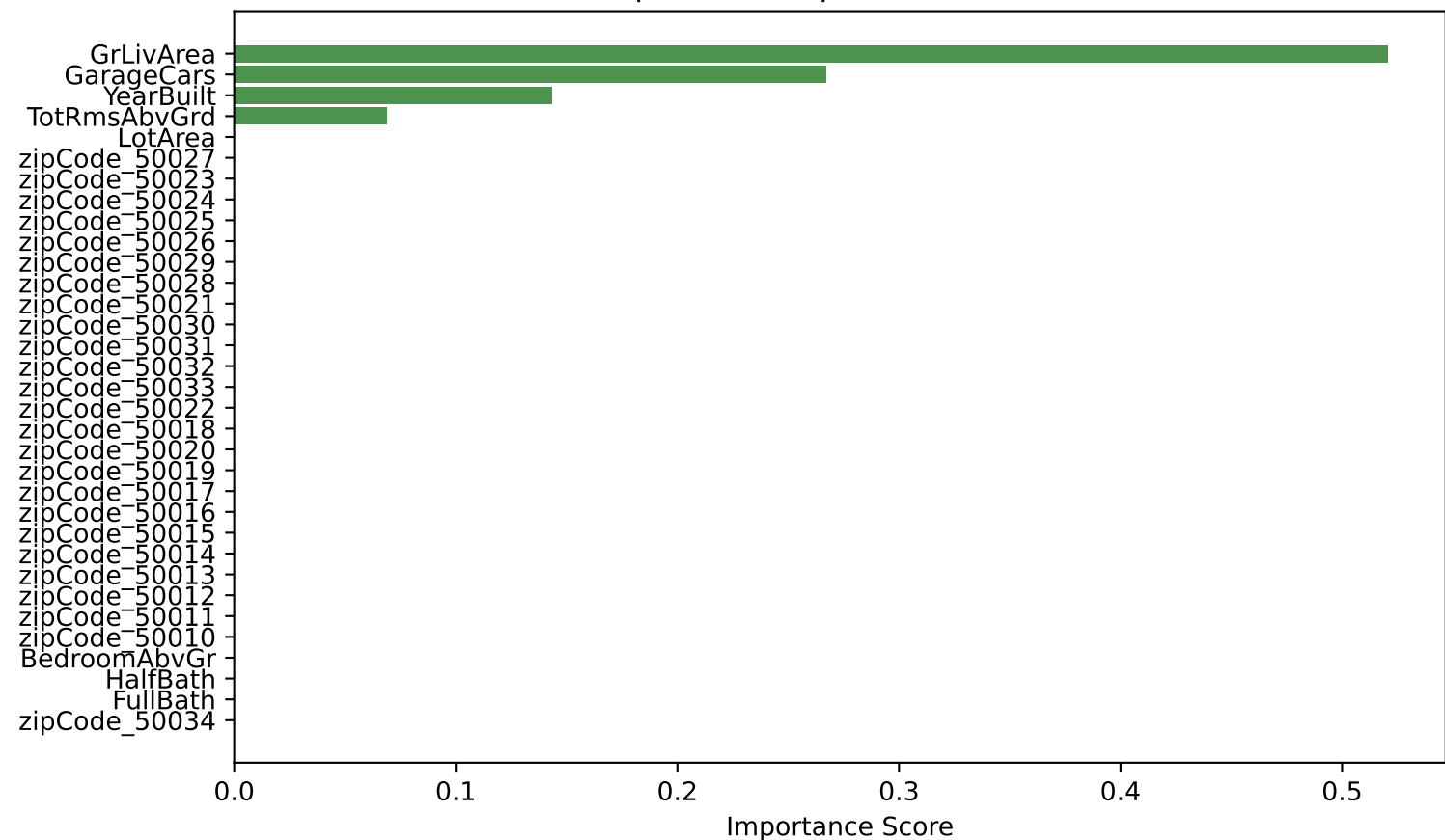
Feature Importance (zipCode One-Hot Encoded)
