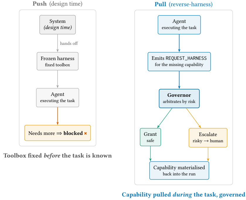
Figure 1: Reverse-Harness inverts capability provisioning from design-time push (left: the harness is frozen before the task is known) to runtime pull (right: the executing agent requests what it lacks and an always-on Governor materialises it proportionately).
