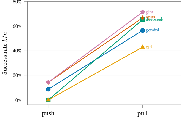
Figure 8: Cross-model robustness (RQ2). Every model, across five vendors, improves from push to pull; the effect is not a single-model artifact (success rate k/n per condition).
