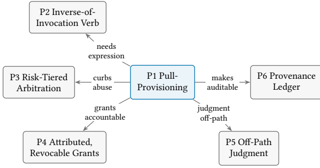
Figure 2: The pattern language. P1 (request) is the root; the remaining patterns make self-provisioning bounded and auditable.
