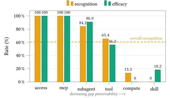
Figure 5: Recognition bounds efficacy (RQ1 \times RQ5). Per family: correct-kind request rate (recognition) and pull-condition success rate (efficacy). Concrete gaps (access, mcp) are recognised and recovered; soft gaps (compute, skill) are neither. Same values as Tables 4 and 9.
