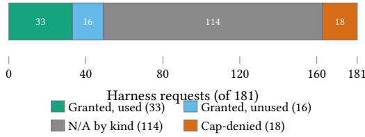
Figure 6: Request-outcome taxonomy (RQ1). The 181 harness requests reconcile to 163 grants (33 used, 16 unused, 114 not-applicable-by-kind) plus 18 over-delegation denials at the per-run cap; no wasted requests, and all 181 decided deterministically. Same values as Table 5.
