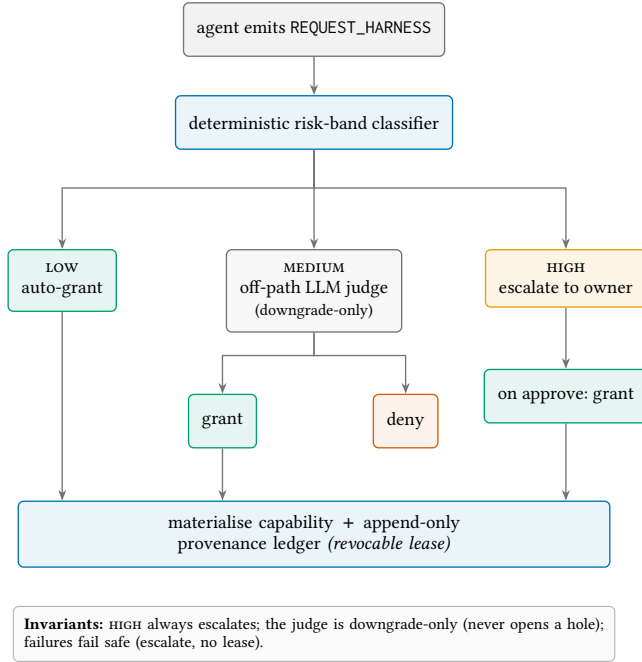
Figure 4: Proportionate governance. Each request is arbitrated by a deterministic risk band — LOW auto-grants, MEDIUM consults a downgrade-only judge, HIGH always escalates to the owner — and every grant is materialised and recorded in an append-only ledger.
