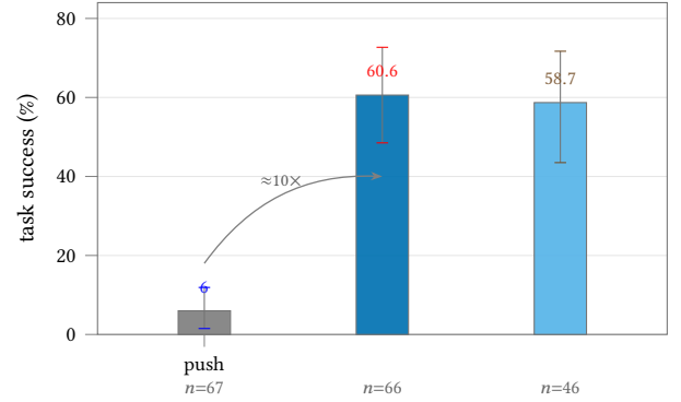
Figure 7: Capability-gap recovery (RQ2). A frozen-harness baseline succeeds on 6.0% of gap-bearing tasks; governed pull on 60.6% (pull-min 58.7%), recovering 60% of baseline failures. Whiskers are 95% bootstrap CIs. Same values as Table 6, generated from paper_numbers.json.
