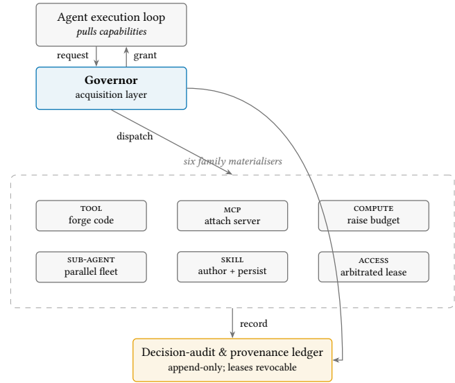
Figure 3: Reference implementation (systemu). The execution loop pulls capabilities through one Governor that dispatches to six family materialisers—covering both synthesis (tool) and attachment (MCP)—and records every grant in an append-only ledger with revocable leases.
