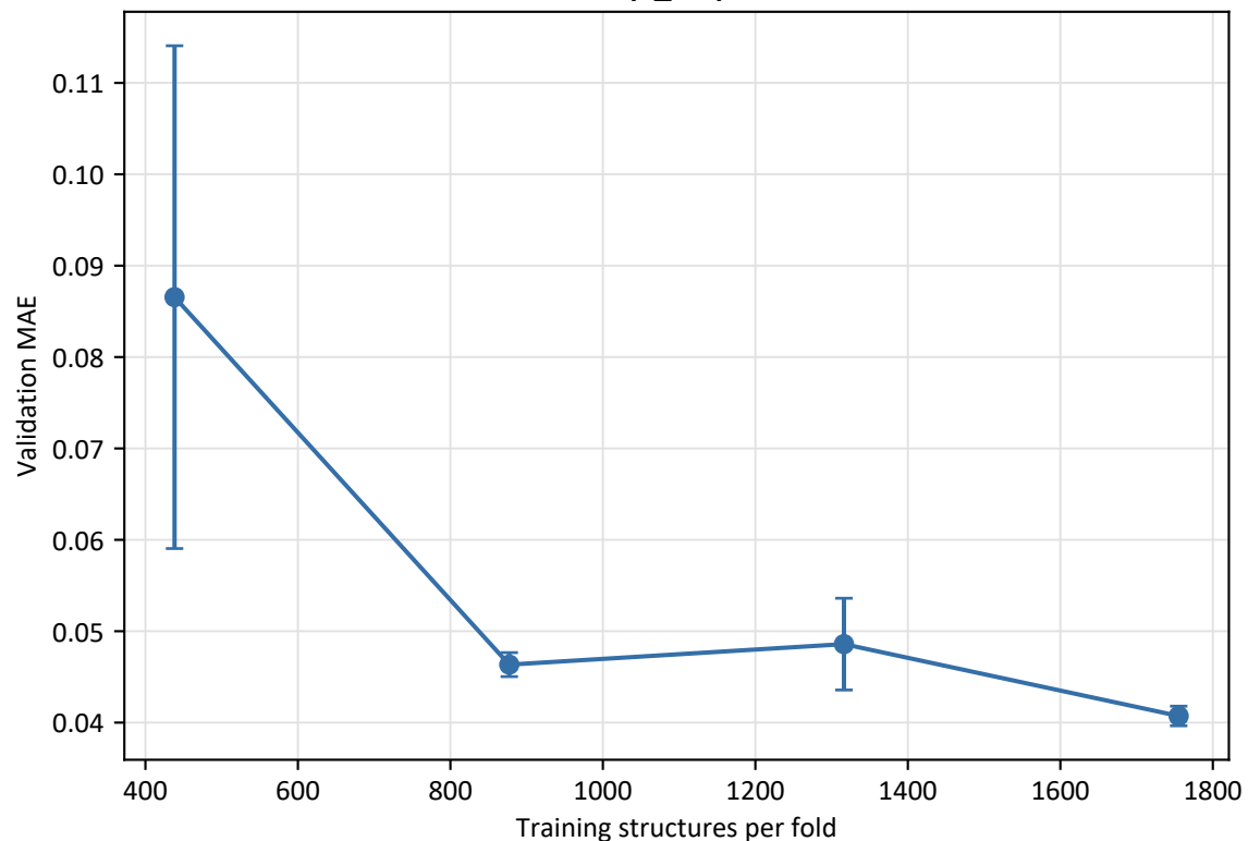
Spin-conserving frontier gap
