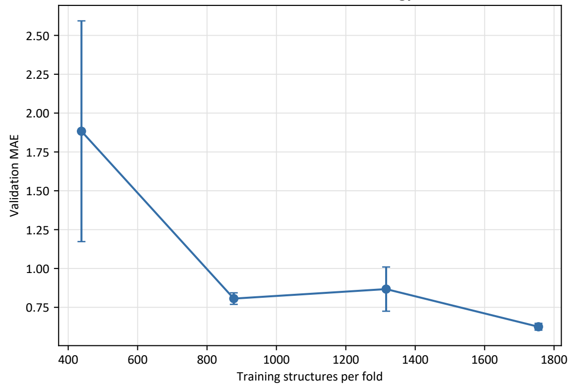
Corrected SOMO-SOMO energy
