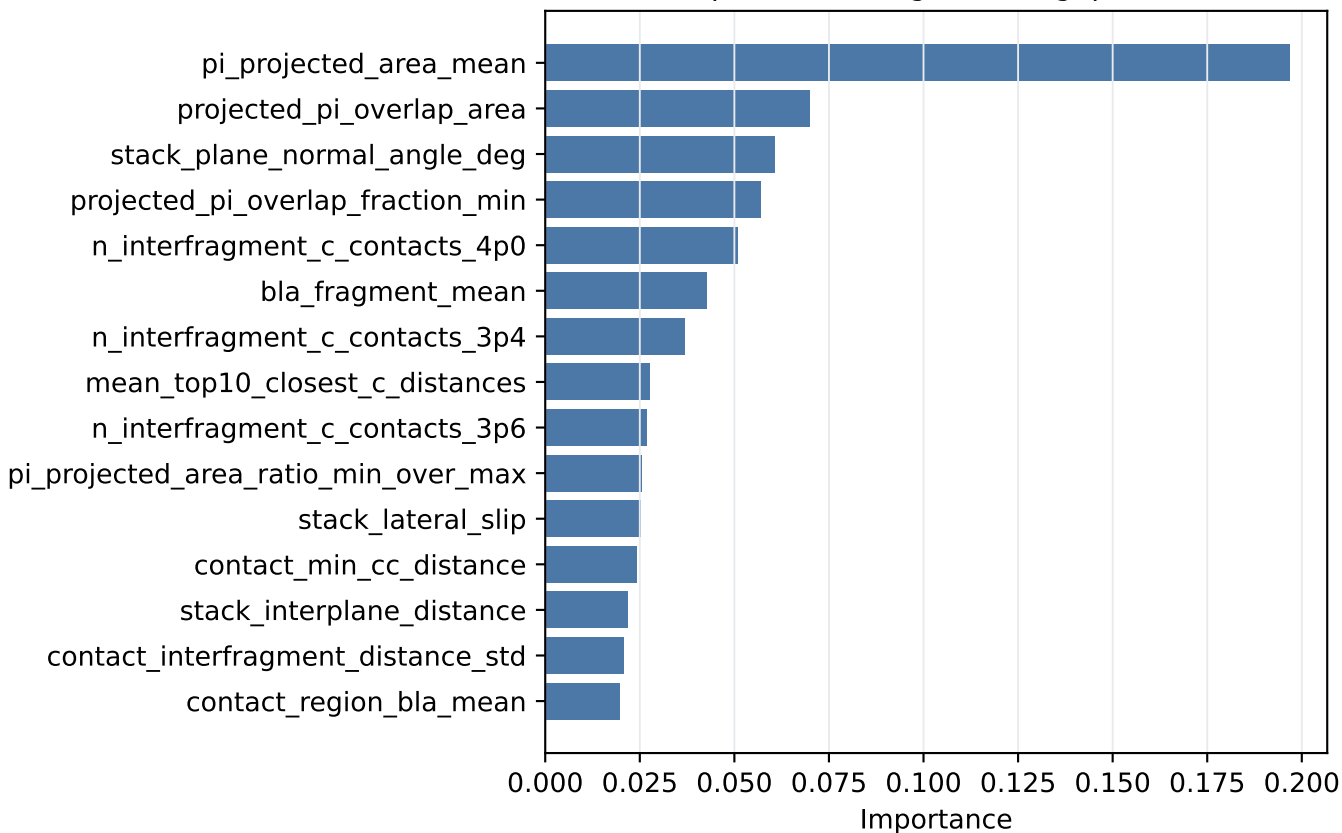
Spin-conserving frontier gap (eV)
