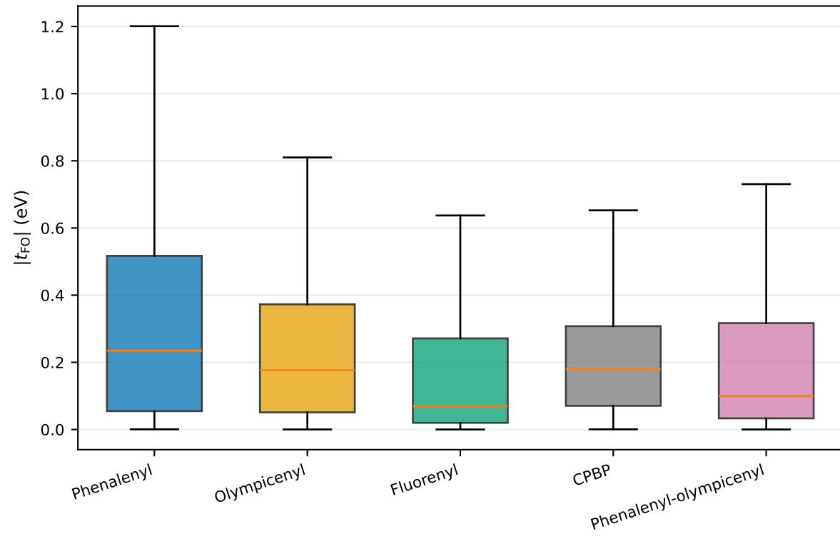
Fragment-orbital SOMO coupling by dimer family
