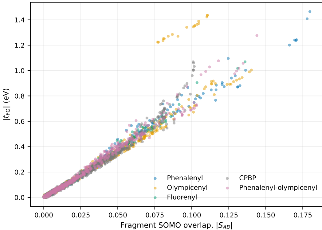
Coupling and fragment-orbital overlap
