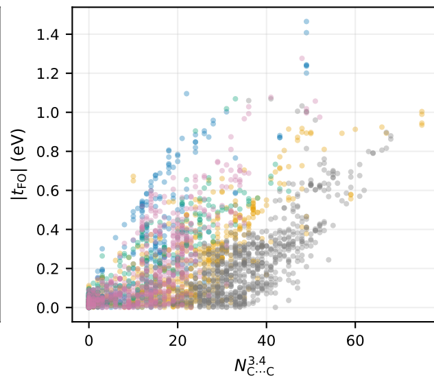
Short C...C contacts ( \rho_s = 0.61 )
