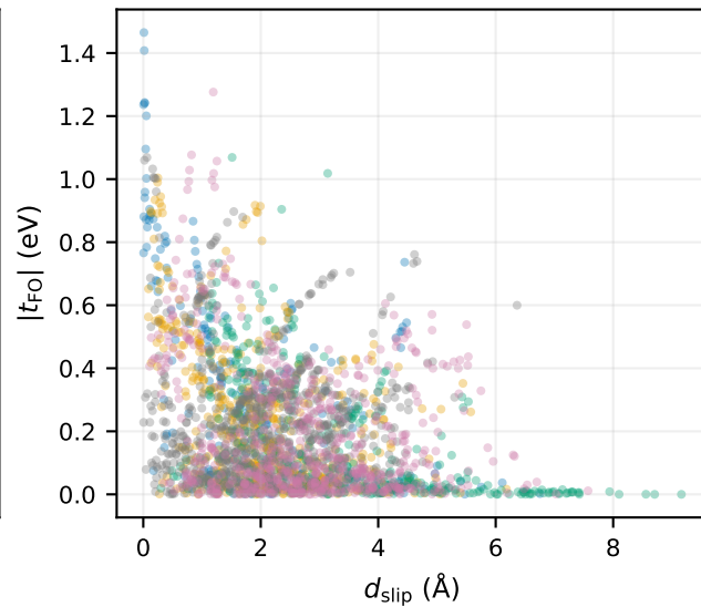
Short C...C contacts ( \rho_s = 0.61 )
