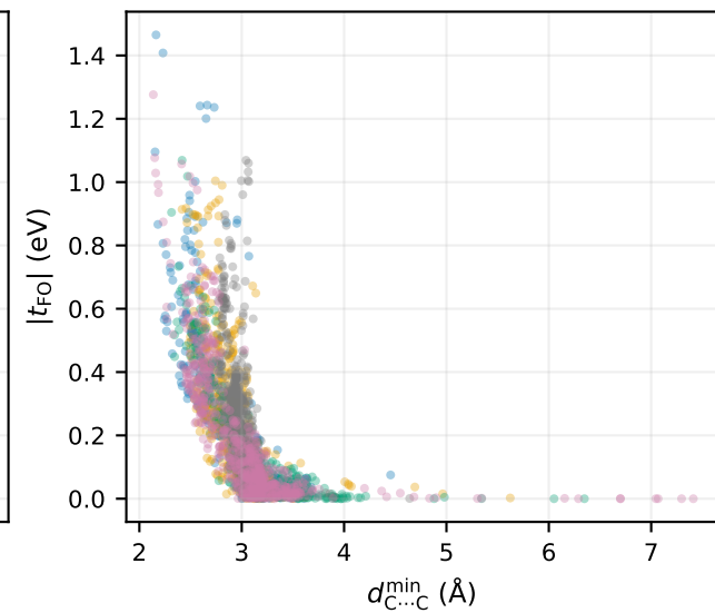
Shortest C...C distance ( \rho_s = -0.84 )
