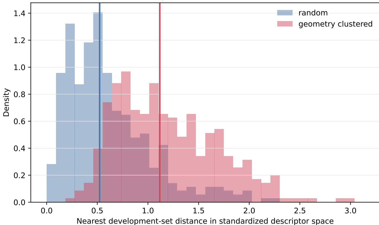
Structural separation of the external test set
