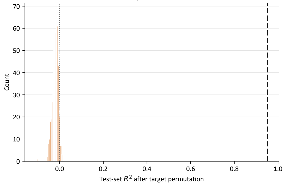
Descriptor-based MLP
