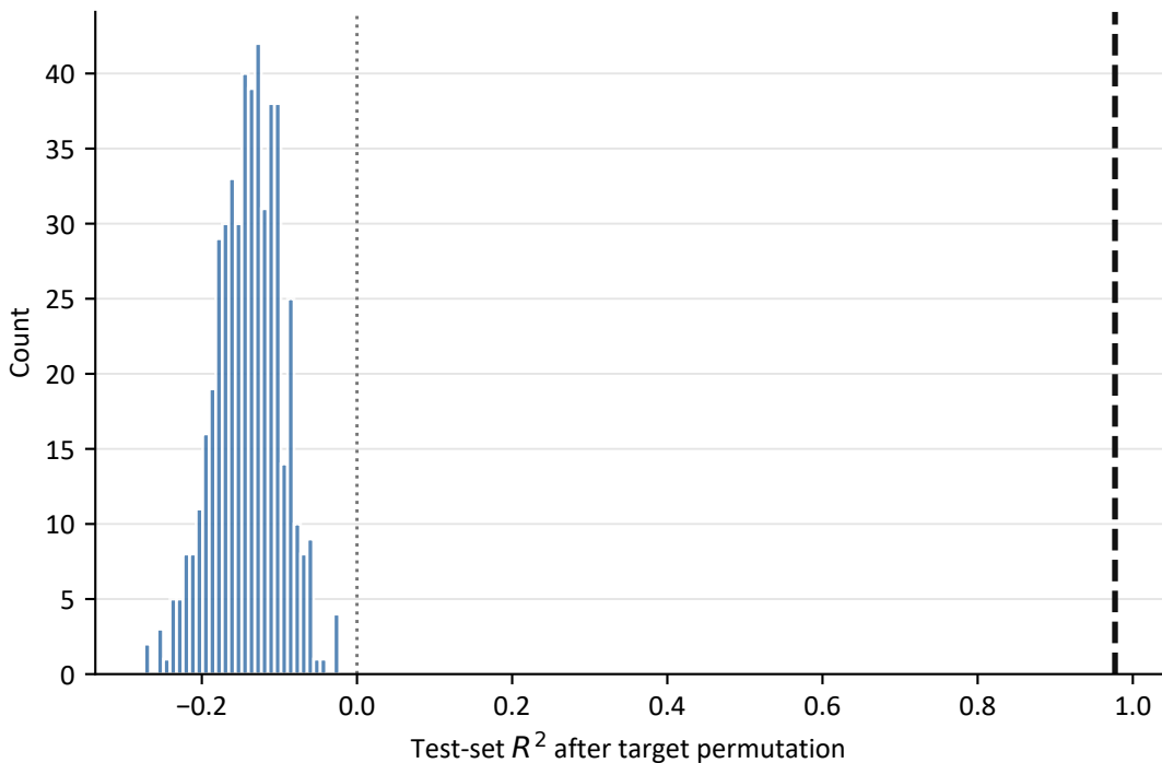
Extra Trees
