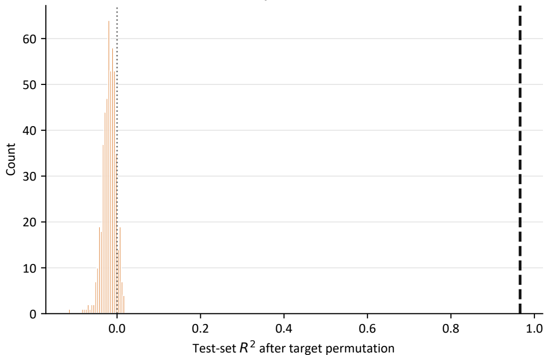
Descriptor-based MLP
